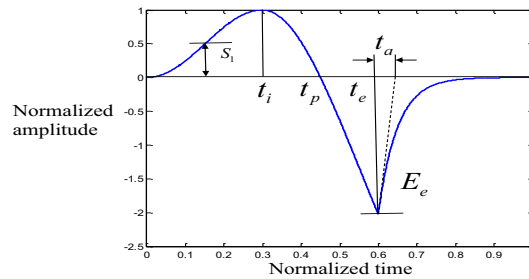
FIGURE 2: An example of the proposed model with S_1 = 0.5 , t_i = 0.3 , t_p = 0.45 , t_e = 0.6 , E_e = 2 , and t_a = 0.05 .
