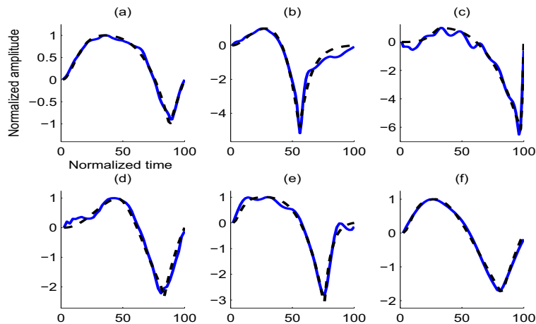
FIGURE 3: Target AbS source pulses and the corresponding least-MSE-fitted sources using the proposed model for six different speakers. Panels (a), (b), and (c): male speakers. Panels (d), (e), and (f): female speakers. Solid line: AbS source. Dashed line: the proposed model.
