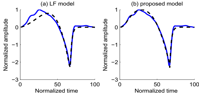
FIGURE 1: An example of fitting the LF and the proposed models to the same AbS source pulse subject to MSE criteria while constraining the models to fit the negative peak of the flow derivative precisely. Solid line: AbS source. Dashed line: model-fitted source.
