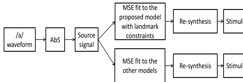
FIGURE 4: Flowchart showing how stimuli were generated for the perceptual experiment.
