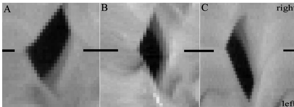
Fig. 8. DKG for the illustrative cases in Figure 7. Glottal midline is designated by the black bars, the top is right vocal fold excursion and the bottom is left vocal fold excursion. (A) Condition left RLN 6 right 0: The left vocal fold led in the opening phase of vibration, but the amplitude of vibration is greater on the right. (B) Condition left RLN 6 right RLN 5: The opening phase and amplitude of vibration are both symmetric. (C) Condition left RLN 0 and right RLN 6: The right vocal fold led in the opening phase of vibration, but the amplitude of vibration is greater on the left. DKG = digital kymograms; RLN = recurrent laryngeal nerves; SLN = superior laryngeal nerve.
